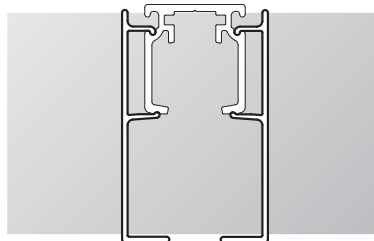
Valance profile - double sided mounting for ceiling mounted systems, single side mounting for wall mounted systems
