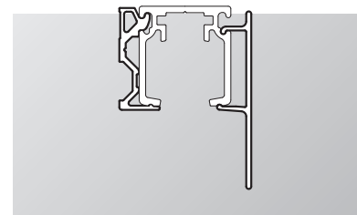
Valance profile - double sided mounting for ceiling mounted systems, single side mounting for wall mounted systems
